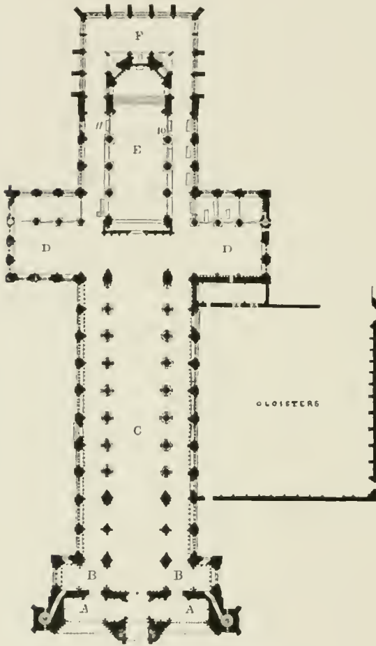
PLAN OF PETERBOROUGH CATHEDRAL. 1
